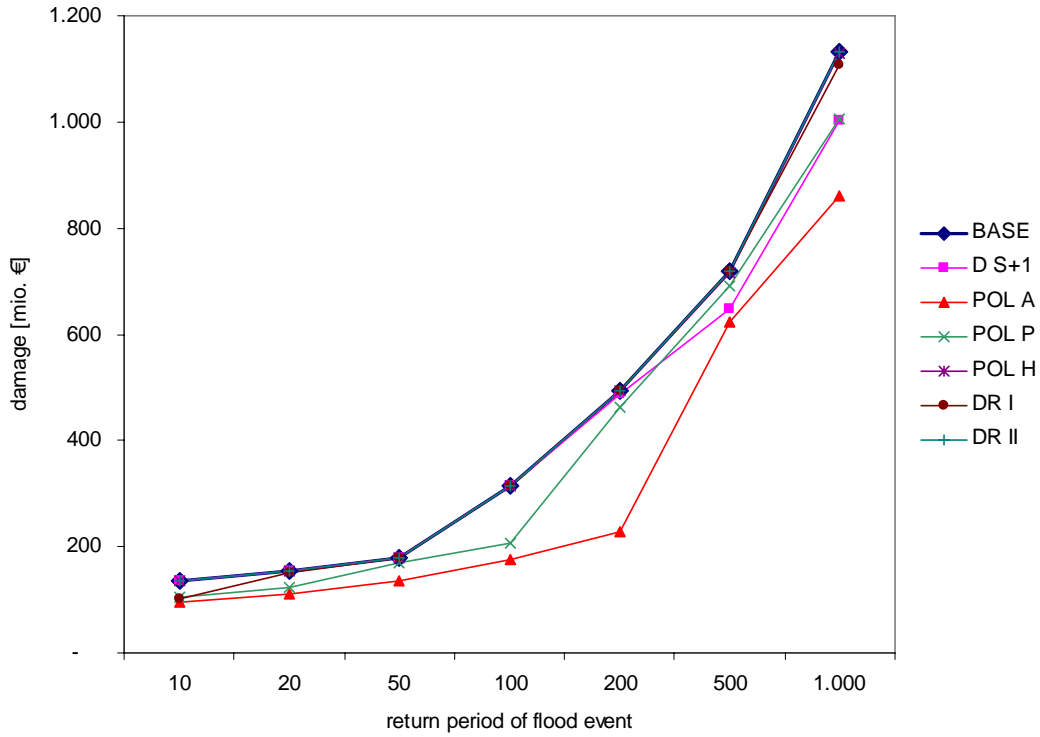
Figure 6: Effect of the assessed mitigation strategies on the flood damage for flood events with increasing recurrence intervals.
